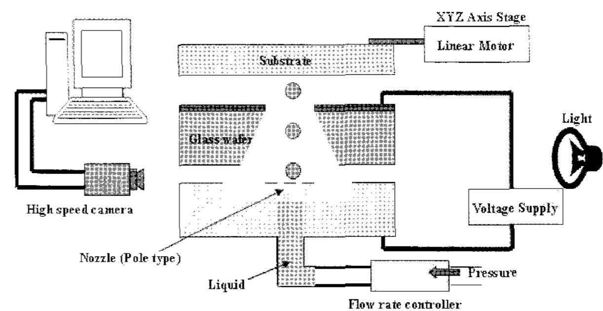
Fig. 11. The schematic of the experimental system.
